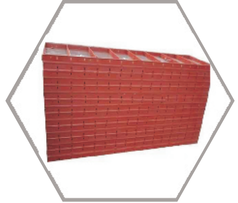
Plywood & Steel Wall Form Panels (PERI Type) PG - 2003
